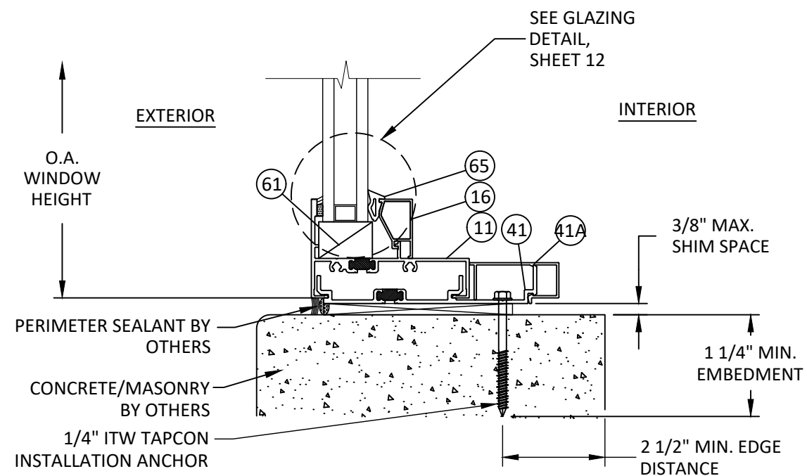
G 7 VERTICAL SECTION FIXED SILL - CONCRETE/MASONRY STRAP ANCHOR - TYP.
